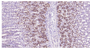
Immunohistochemical analysis of paraffin embedded Mouse stomach tissue slide using IHC0551M (Mouse GRP94 Kit).
