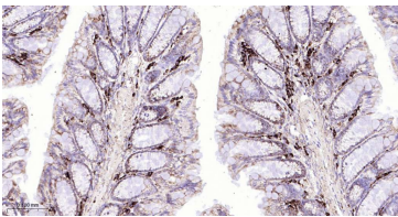
Immunohistochemical analysis of paraffin embedded Mouse colon tissue slide using IHC0551M (Mouse GRP94 Kit).
