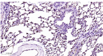
Immunohistochemical analysis of paraffin embedded Mouse lung tissue slide using IHC0518M (Mouse Lysozyme Kit).
