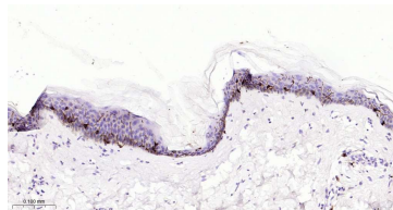
Immunohistochemical analysis of paraffin embedded Human skin tissue slide using IHC0517H (Human CD207 Kit).
