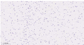
Immunohistochemical analysis of paraffin embedded Human brain tissue slide using IHC0517H (Human CD207 Kit).
