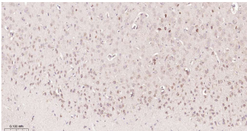
Immunohistochemical analysis of paraffin embedded Rat brain tissue slide using IHC0515R (Rat STAT6 Kit).
