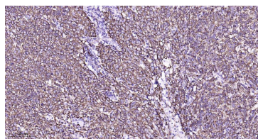
Immunohistochemical analysis of paraffin embedded Human thyroid carcinoma tissue slide using IHC0503H (Human Cytokeratin 8 Kit).
