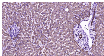
Immunohistochemical analysis of paraffin embedded Human liver tissue slide using IHC0503H (Human Cytokeratin 8 Kit).
