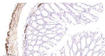
Immunohistochemical analysis of paraffin embedded mouse colon tissue slide using IHC0458 (Hsp27 IHC Kit).
