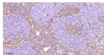
Immunohistochemical analysis of paraffin embedded human colon cancer tissue slide using IHC0458 (Hsp27 IHC Kit).
