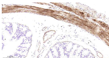
Immunohistochemical analysis of paraffin embedded rat colon tissue slide using IHC0458 (Hsp27 IHC Kit).
