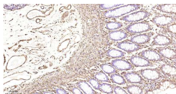
Immunohistochemical analysis of paraffin embedded human colon tissue slide using IHC0458 (Hsp27 IHC Kit).
