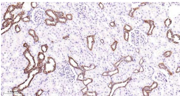
Immunohistochemical analysis of paraffin embedded rat kidney tissue slide using IHC0424R (Rat Hexokinase 1 IHC Kit).
