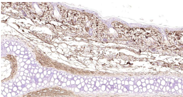
Immunohistochemical analysis of paraffin embedded rat skin tissue slide using IHC0401R (Rat Lumican IHC Kit).
