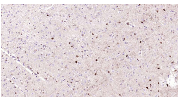
Immunohistochemical analysis of paraffin embedded rat brain tissue slide using IHC0386 (BLBP Kit).
