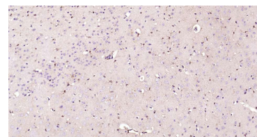
Immunohistochemical analysis of paraffin embedded mouse brain tissue slide using IHC0386 (BLBP Kit).
