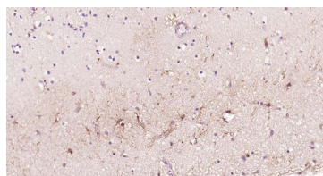
Immunohistochemical analysis of paraffin embedded human brain tissue slide using IHC0386 (BLBP Kit).
