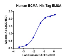
Immobilized Human BCMA, His Tag at 0.5ug/ml (100ul/Well). Dose response curve for Human BAFF, Fc Tag with the EC50 of 18.2 ng/ml determined by ELISA.
