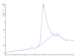
The purity of BCMA is greater than 95% as determined by SEC-HPLC.
