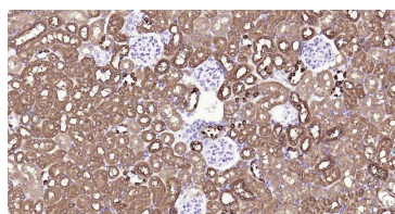
Immunohistochemical analysis of paraffin embedded mouse kidney tissue slide using IHC0297M (Mouse ALDH1L1 IHC Kit).
