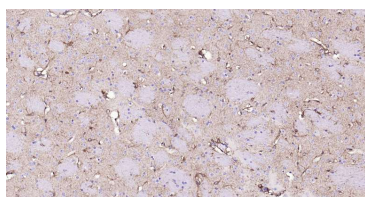
Immunohistochemical analysis of paraffin embedded mouse brain tissue slide using IHC0297M (Mouse ALDH1L1 IHC Kit).
