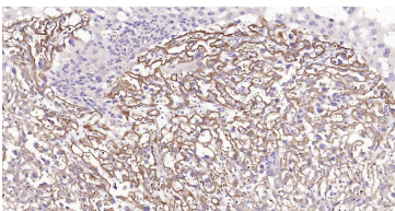
Immunohistochemical analysis of paraffin embedded mouse placenta tissue slide using IHC0203M (Mouse TFRC IHC Kit).
