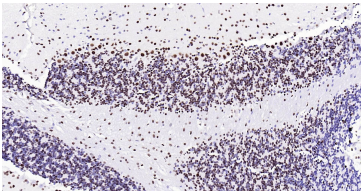
Immunohistochemical analysis of paraffin embedded mouse cerebellum tissue slide using IHC0177M (Mouse TARDBP IHC Kit).
